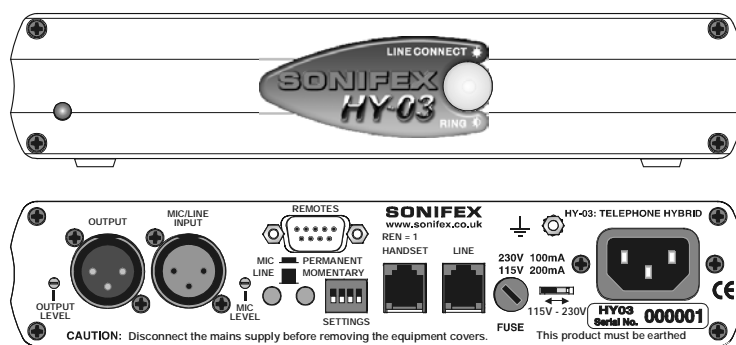
Figure 1-1 : HY-03 & HY-03 US Front & Rear
