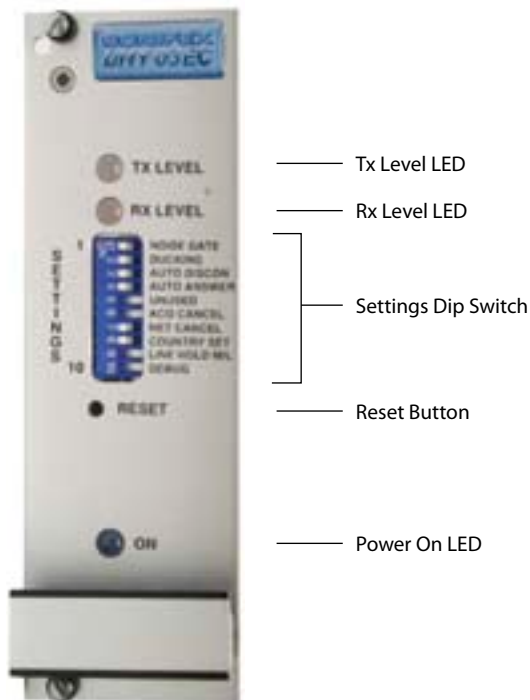
Figure 2-6 : DHY-03EC Controls.
