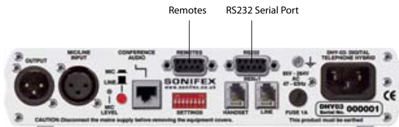
Figure 2-4 : Rear Panel Controls.
