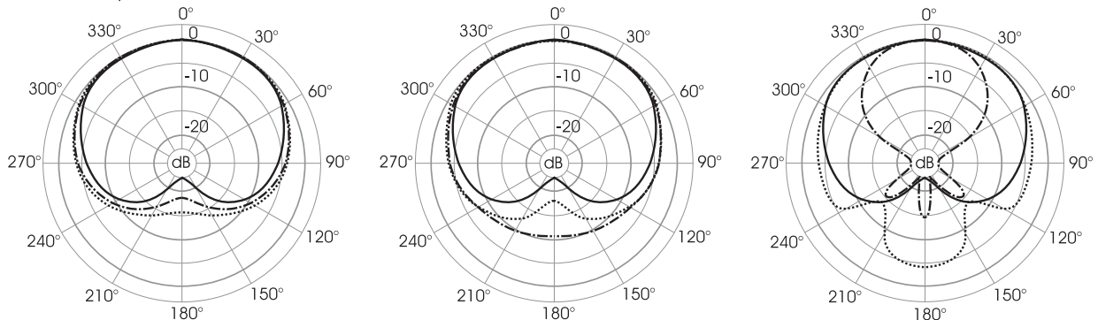
Polar patterns M 1030
