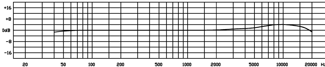
Frequency response curve ± 2.5 dB 0 dB \triangleq 30 mV/Pa MC 837
