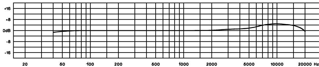
Frequency response curve ± 2.5 dB 0 dB \triangleq 30 mV/Pa MC 836
